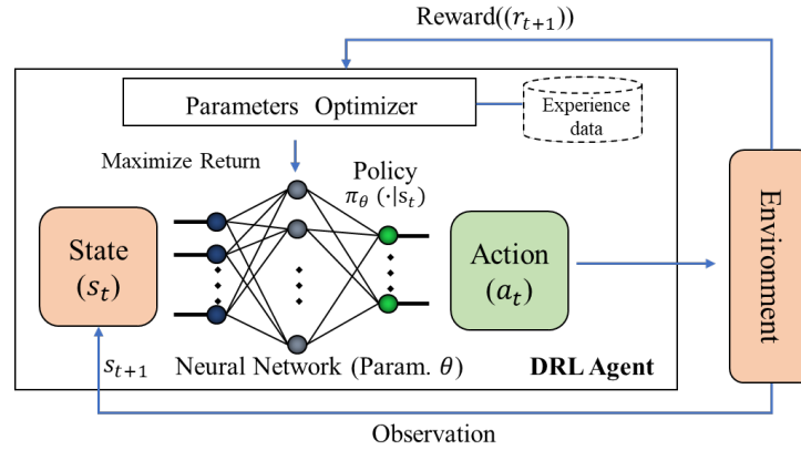
Fig. 2. The semantics of deep reinforcement learning.
